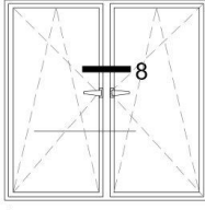
BİNLİ İÇE AÇILIR ORTA KAYITLI DETAY OVERLAPPING INWARD OPENING DETAIL WITH MULLION
