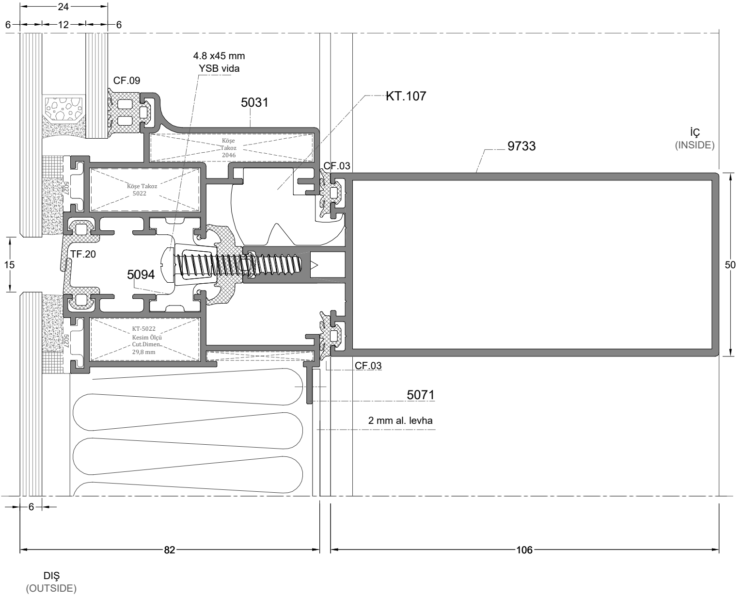
DETAY 4 DETAIL 4
