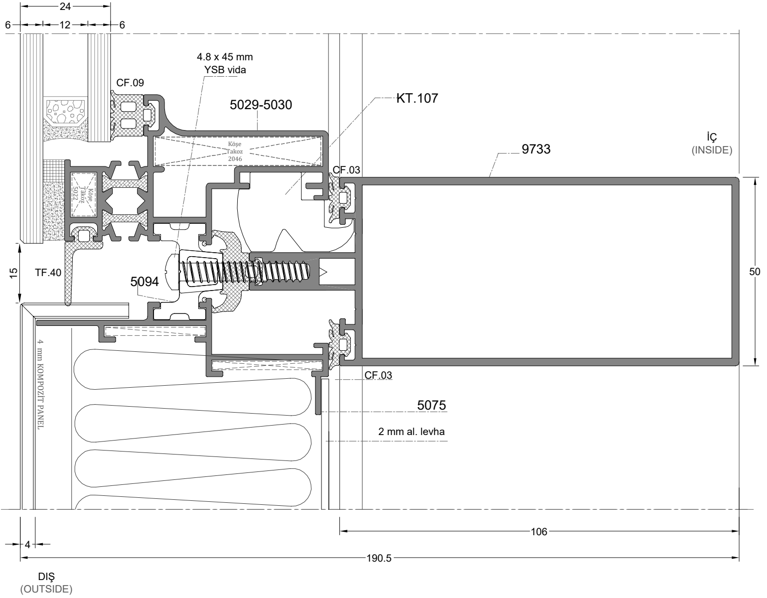
DETAY 6 DETAIL 6
