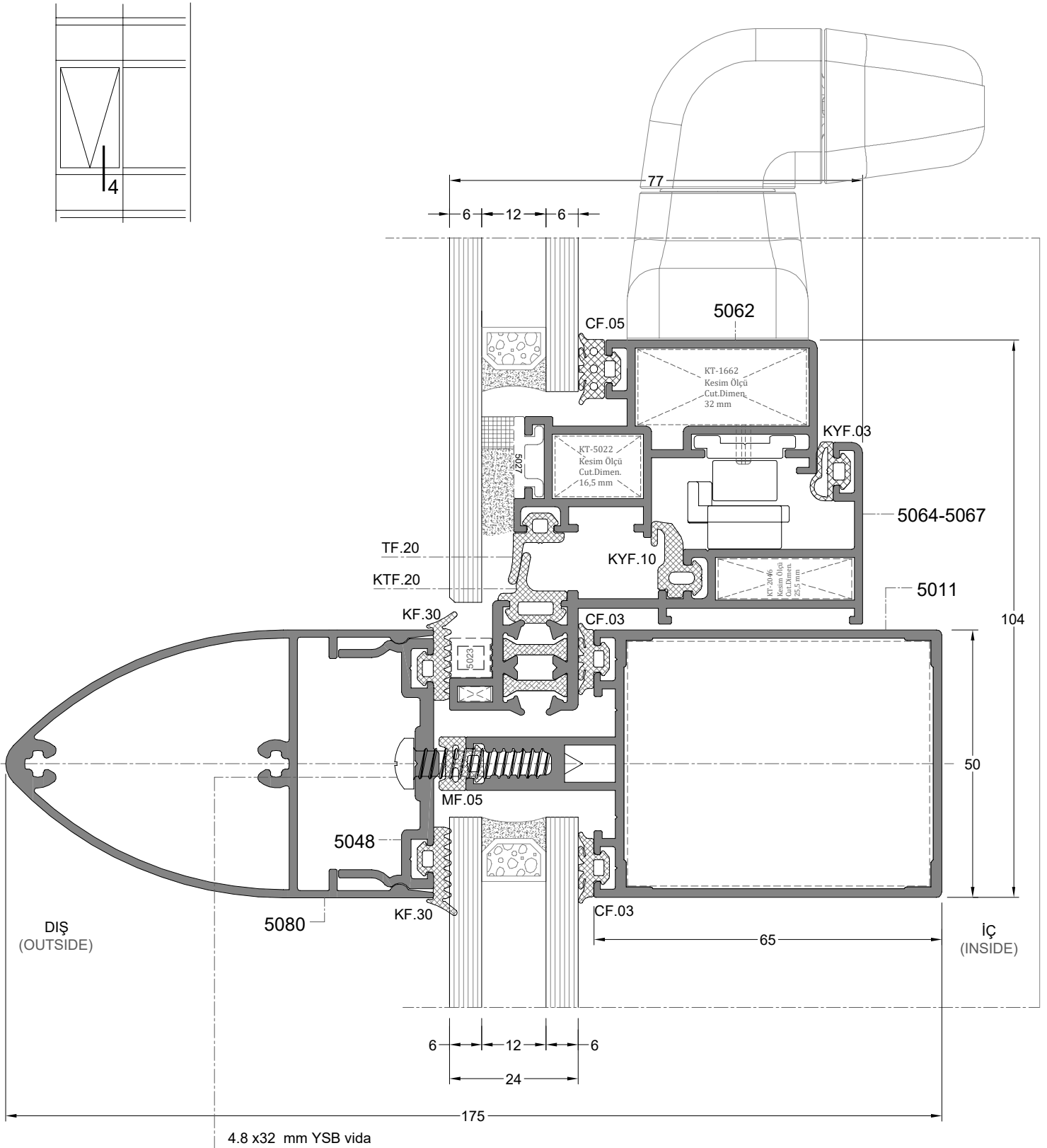
DETAY 4 DETAIL 4
