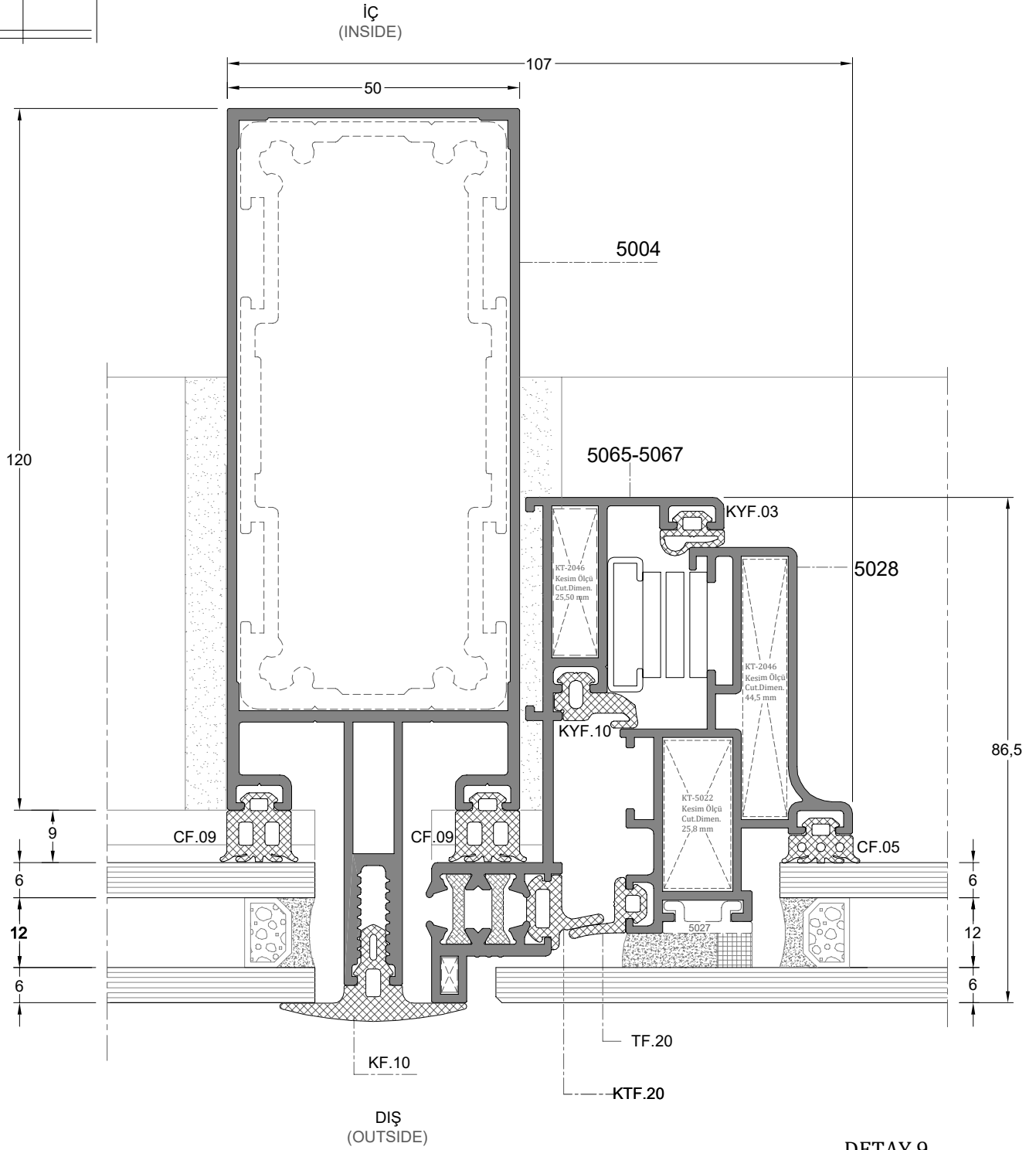
DETAY 9 DETAIL 9
