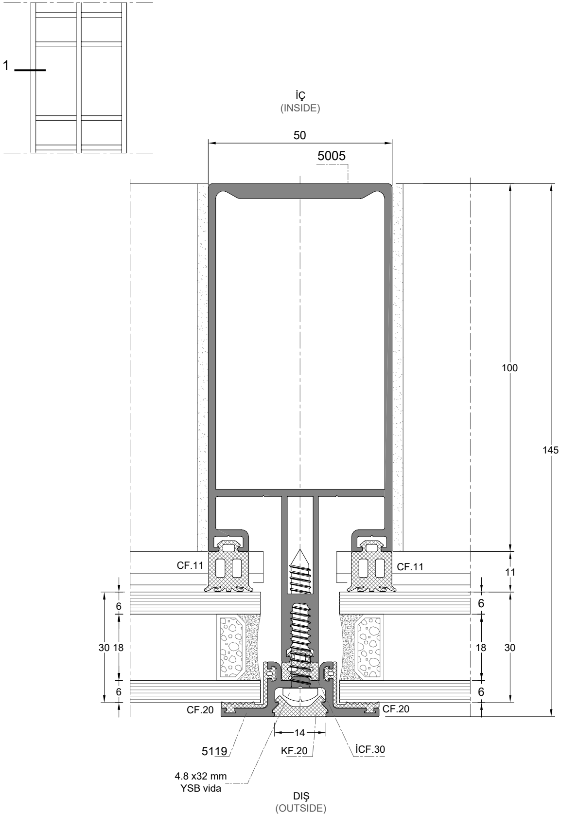
DETAIL 1 DETAIL 1
