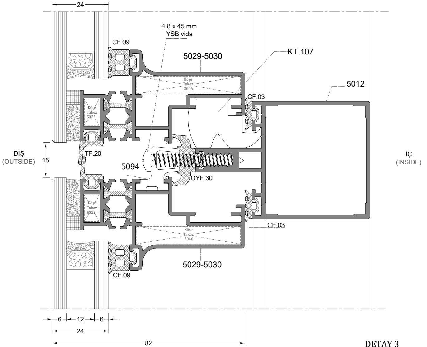
DETAY 3 DETAIL 3
