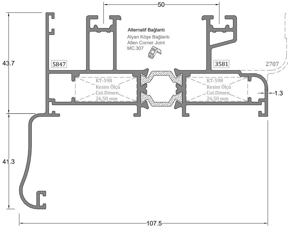
İki Raylı Kasa Profili DOUBLE RAIL FRAME PROFILE
