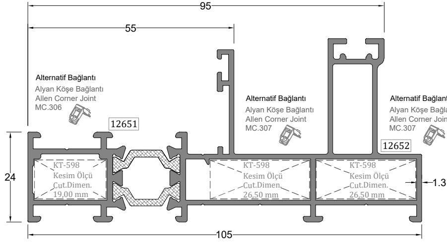
Tek Raylı Kasa Profili MONORAIL FRAME PROFILE
