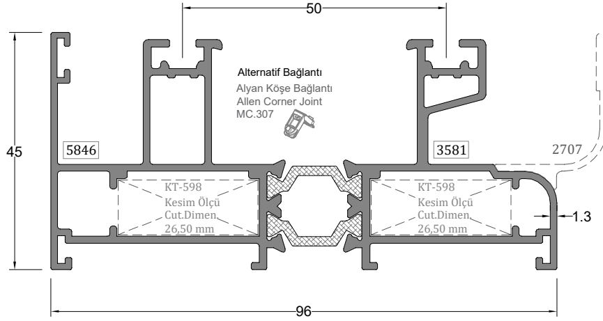
İki Raylı Kasa Profili DOUBLE RAIL FRAME PROFILE
